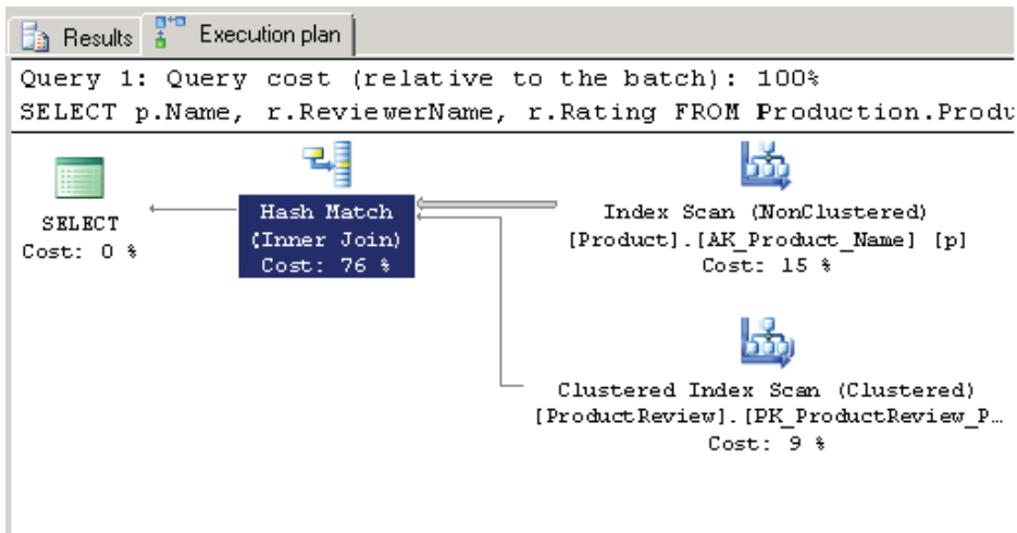
Figure 22-2. A hash join operation
